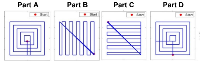
Figure 1: Toolpaths used in Experiment I
